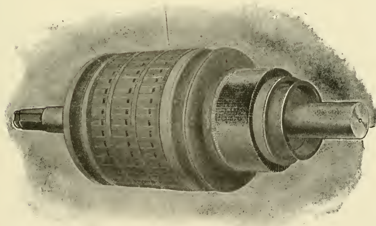
Fig. 39. Armature Complete
